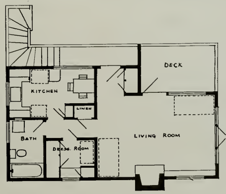
A PARTMENT FLOOR PLAN.
