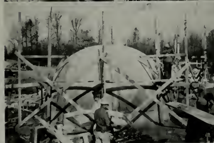
Construction methods: Pictured from top down—(1) Laying out the balloon form; (2) Method of anchoring; (3) Inflating canvas with compressed air; (4) Mounting window frames and dusting balloon so cement won't stick to it.
