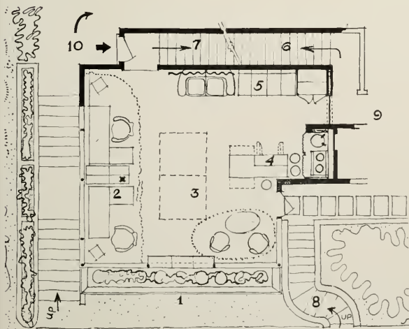
PROPOSED PLAN OF INTERMEDIATE FLOOR FOR RESIDENTIAL OFFICE
