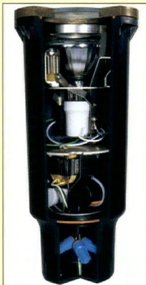
Precision 2 In-grade Fixture (cutaway view)
