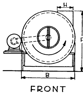
Fig. 3. Plans and chart below may be used to determine the space required for blower room
