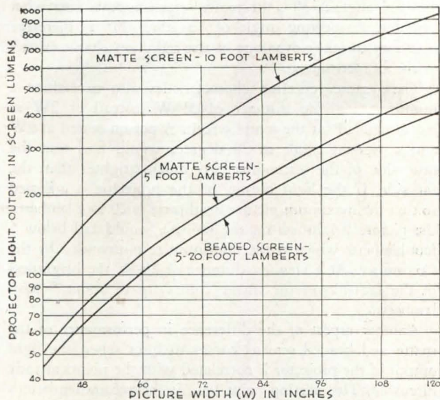
Chart showing maximum picture widths for any given projector light output for either matte or beaded screen
