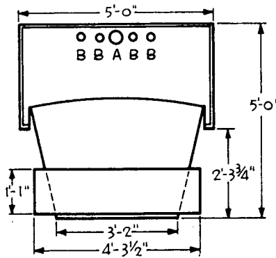
Fig. 2. Plan of organ console. The average organ console is about 4 ft. 3 in. high. An organ having more than three manuals requires 3 in. additional height for each manual added
