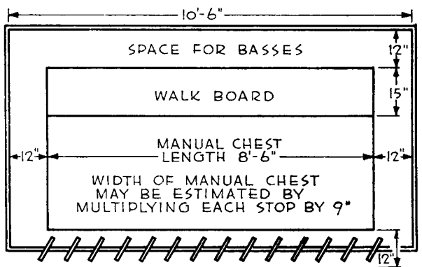
Fig. 1 Above plan is one section of total organ shown below
