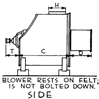
Fig. 3. Plans and chart below may be used to determine the space required for blower room
