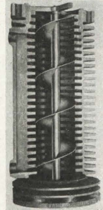
Cutaway of temperature control unit shows cooling fins, helicoid flighting
