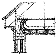
SECTION "A"
