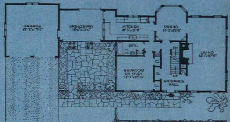
FIRST-FLOOR PLAN graphically shows how rooms are arranged around the center entry hall to make housework easier, and maintain the privacy of each room. Deliveries are made through breezeway to kitchen.
