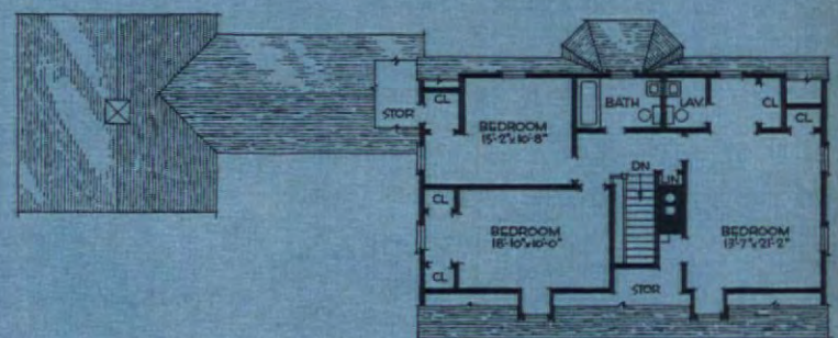
SECOND-FLOOR PLAN has three large bedrooms. Each room has plenty of closet space and dressing area. There are 1½ baths (back-to-back for economy) that can be easily expanded to make two. All bedrooms have cross-ventilation.
