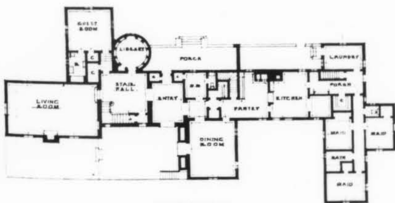
FIRST FLOOR PLAN The main floor plan
