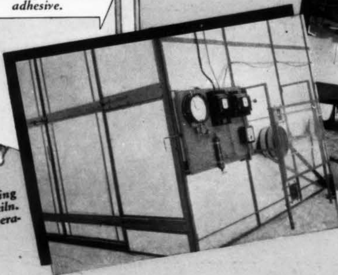
2" Cemesto bolted to steel battens forms the walls of this bakery dough-room. Batten strips are bolted to metal angles at top and bottom.
