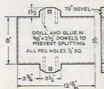
HALF-PATTERN OF BOTTOM ( \frac{3}{4} " REDWOOD)
