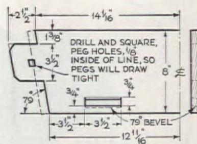
HALF-PATTERN OF SIDES ( \frac{3}{4} " REDWOOD, 2 REQ.)
