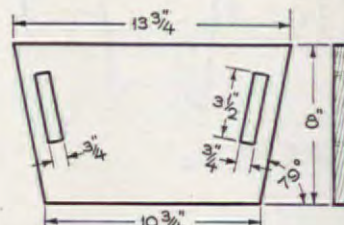
END ( \frac{3}{4} " REDWOOD, 2 REQ.)
