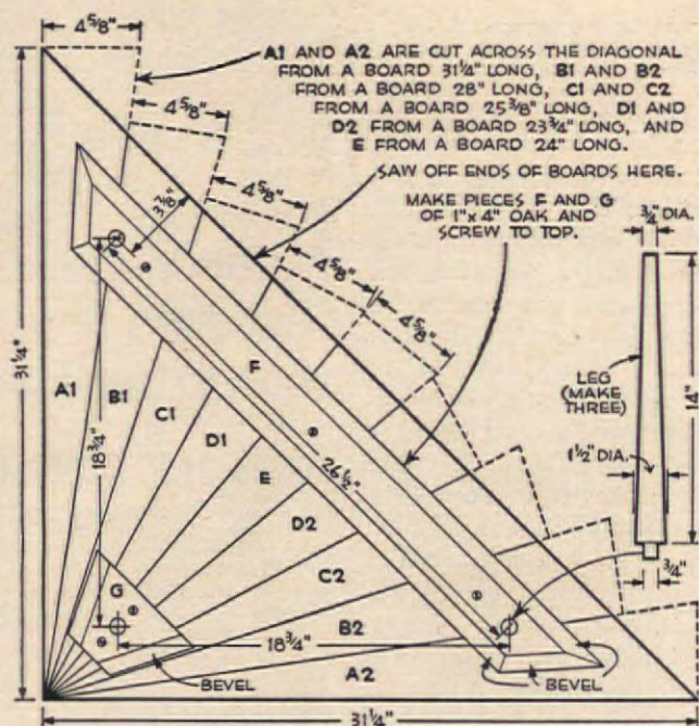
Sketch of underside of table shows sizes and position of pieces.
