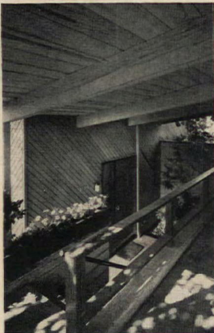
Carport roof connects with house and protects the entrance during rainy weather. It is six steps down from carport to the front door and main level of house.
