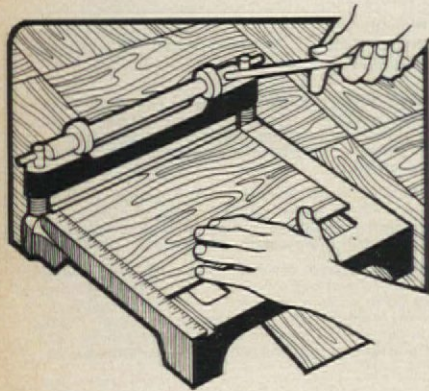
Resilient floor tile cutter
