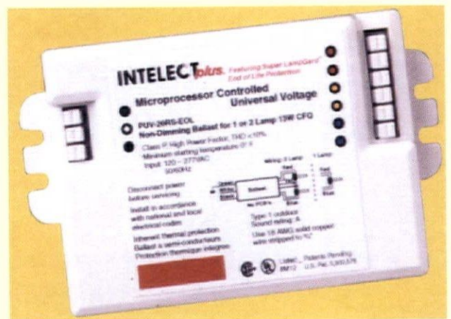
Prescolite's exclusive Intelectplus Electronic Dimming Ballast
