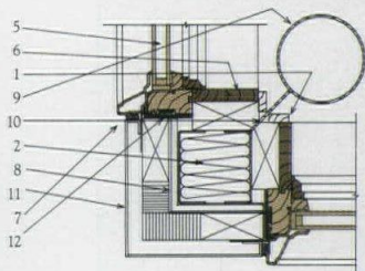
OUTSIDE CORNER DETAIL
