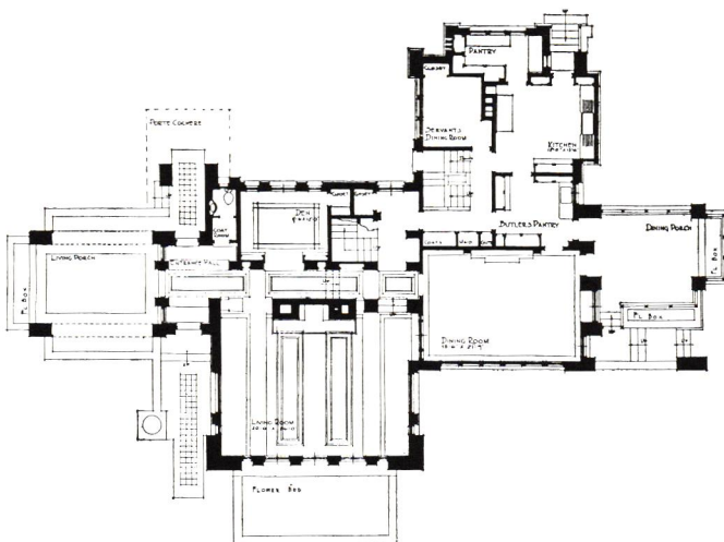
The Robert Mueller house and its plan are shown here. It is located on Millikin Place in Decatur a few doors from the Adolph Mueller house. Frank Lloyd Wright's house for the Irving family is located between the two Mueller houses. Plan from the Architectural Record. Photo courtesy of the New-York Historical Society, New York City.
