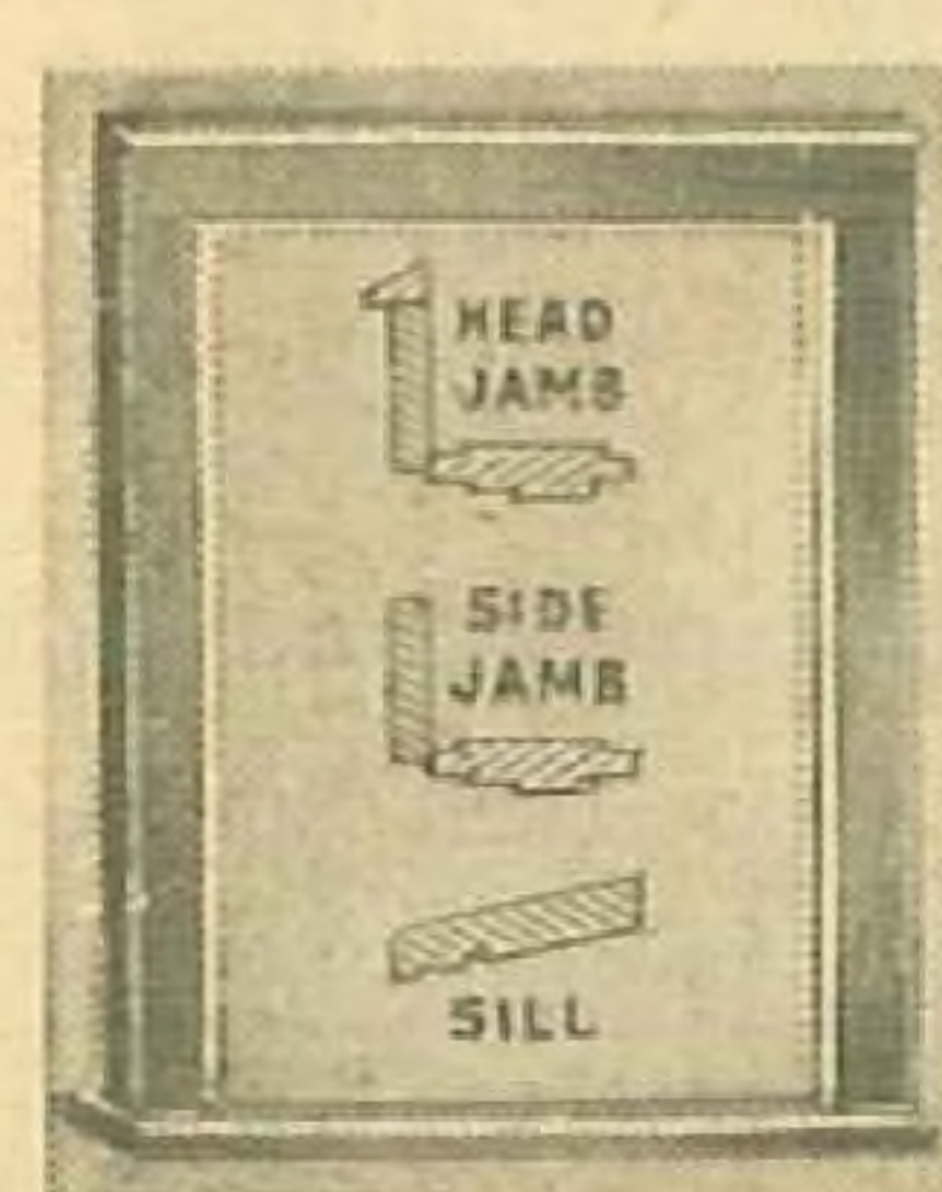
Detail of French Window Frame.
