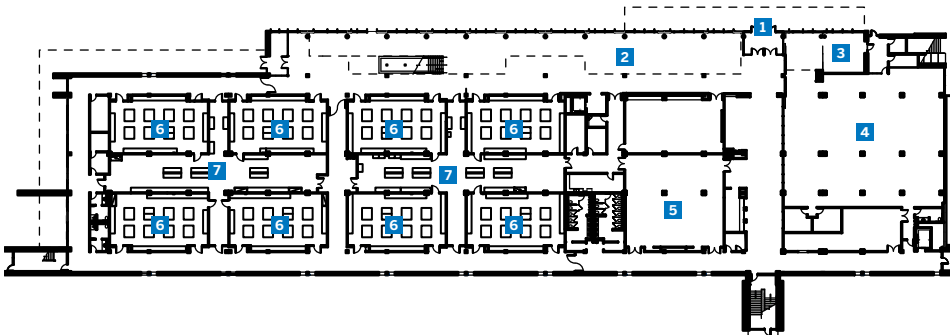
FIRST FLOOR 1 MAIN ENTRY 2 ATRIUM 3 COFFEE AREA 4 BOOK STORE 5 CONFERENCE 6 LAB 7 LAB PREP
