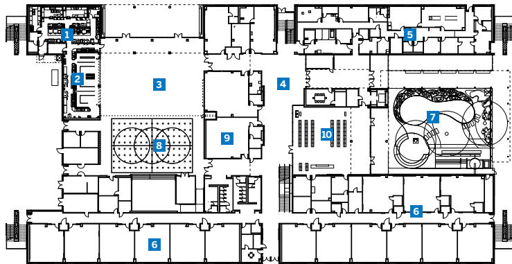
FIRST FLOOR 1 KITCHEN 2 SERVING LINE 3 DINING 4 LOBBY/COMMONS 5 ADMINISTRATION 6 CLASSROOMS 7 ECO POND 8 GYM 9 MUSIC 10 LIBRARY
