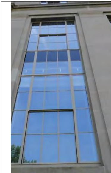
Pilkington NA's vacuum insulated glass was used as part of a restoration project.
